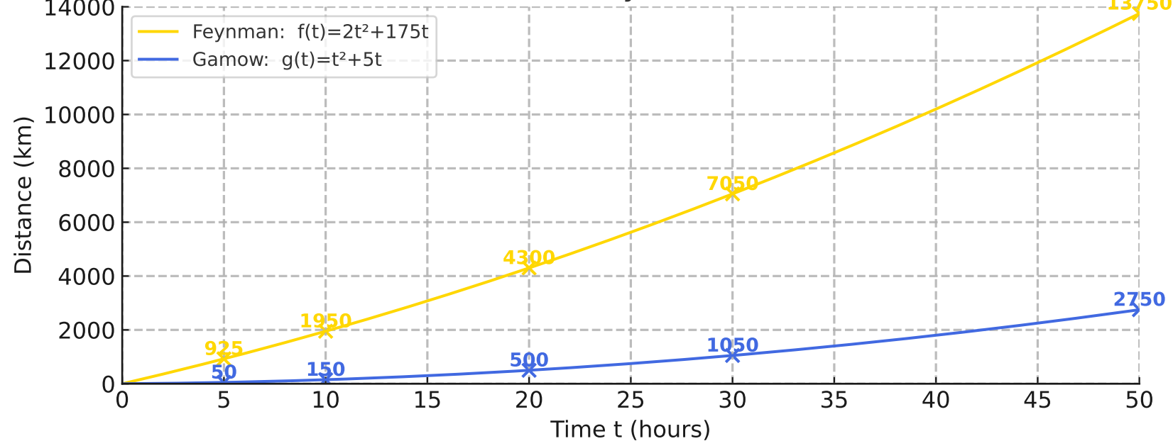
Distance from Earth: Feynman & Gamow Probes
